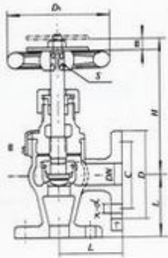
Marine Bronze Angle Valves JIS F7304 16K
