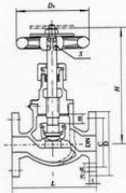
Marine Bronze Globe Valves JIS F7303 16K
